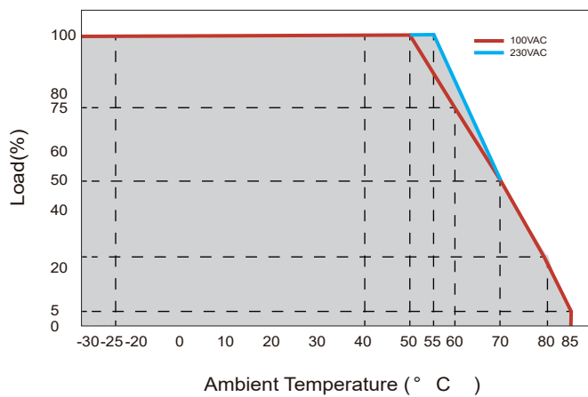
Derating Curve
